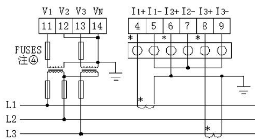
3P3L/2PT+2CT-2 (仪表设置为3P3L-3CT) 注③
