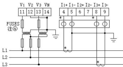
3P3L/2PT+2CT-1 (仪表设置为3P3L-2CT)
