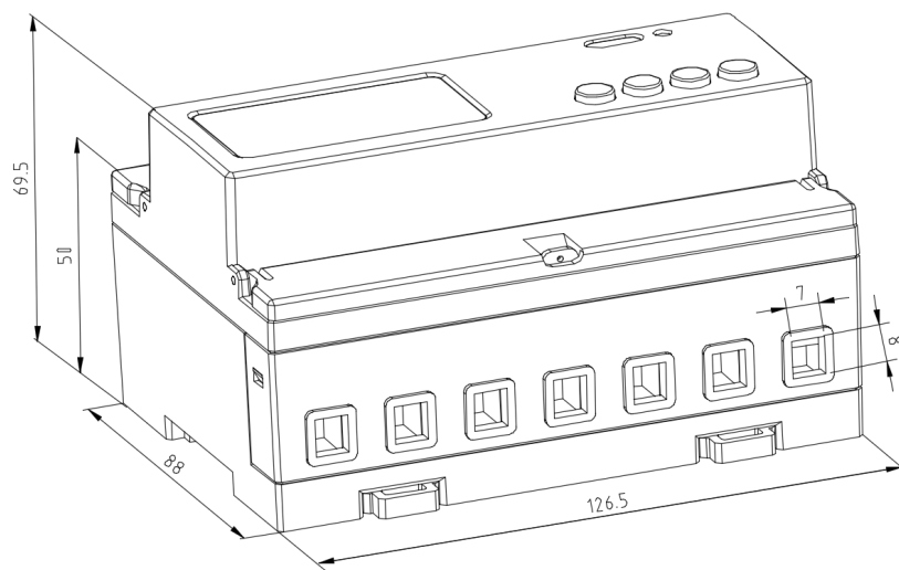
Fig2 direct connect
