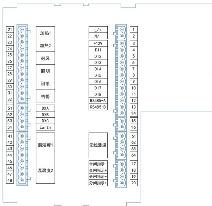
图 1.15 ASD320 背面端子图 Figure 1.15 ASD320 back terminal diagram
