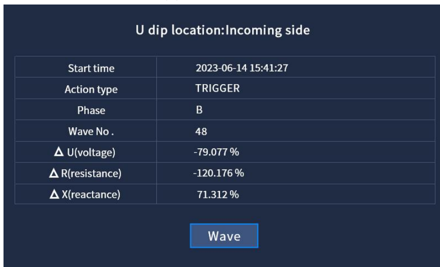
Fig. 4.25(a) Voltage dip location:incoming side
