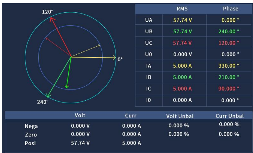
Fig. 4.8 Phasors
