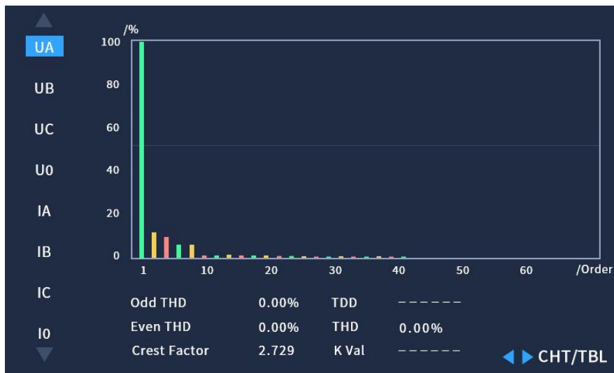
Fig. 4.13 Harmonics Chart
