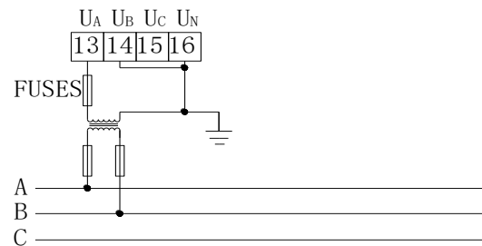
三相三线1PT 3-phase 3-wire 1PT
