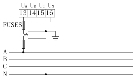
三相四线1PT 3-phase 4-wire 1PT
