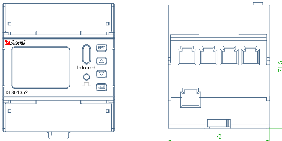
Figure 2 DTSD1352 - 4S dimension
