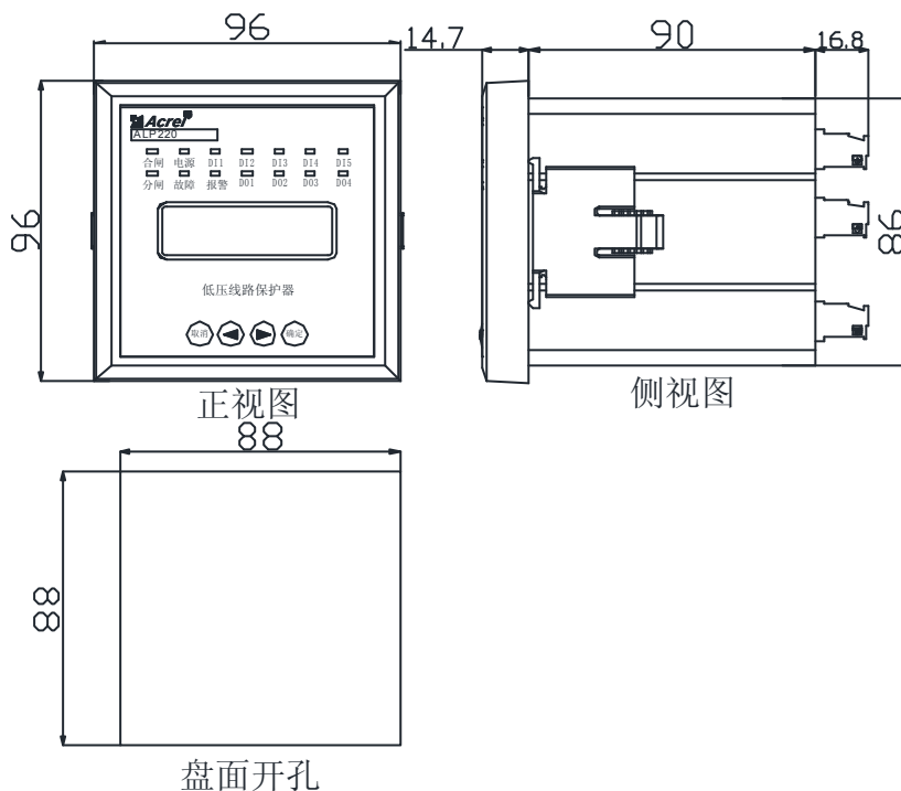
图 2 ALP220 控制模块外形及安装尺寸 Figure 2 Outline and installing dimension of ALP220 control module
