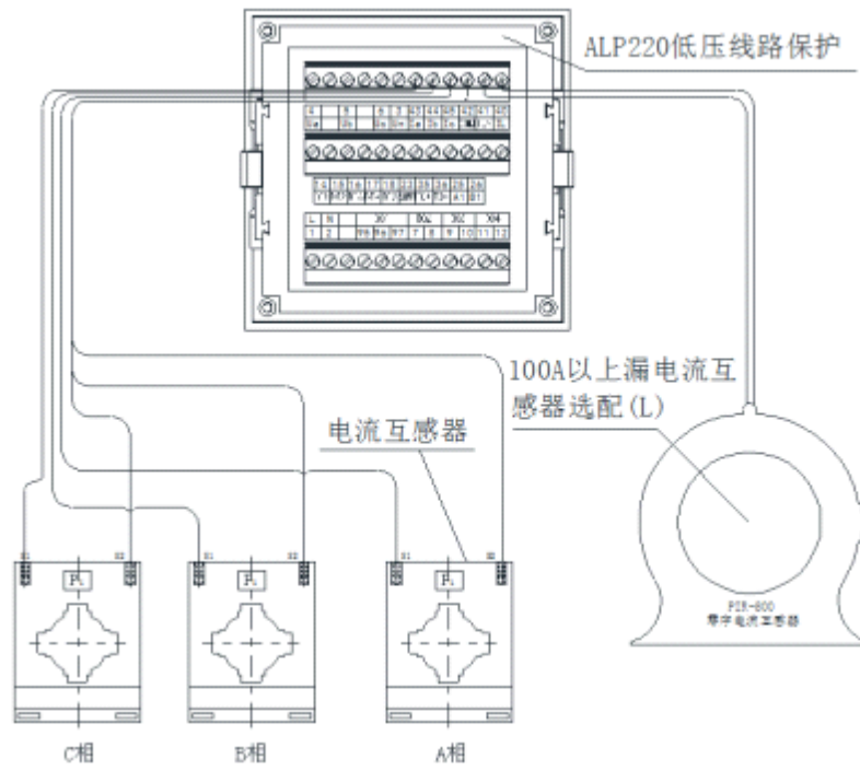
图 17 ALP220-160A、ALP220-400A 产品组成 Figure 17 Product composition of ALP220-160A, ALP220-400A
