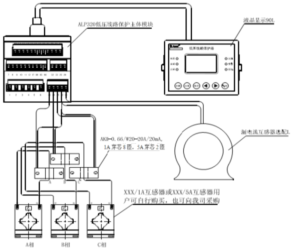
图 18 ALP320-1A、ALP320-5A 产品组成 Figure 18 Product composition of ALP320-1A, ALP320-5A
