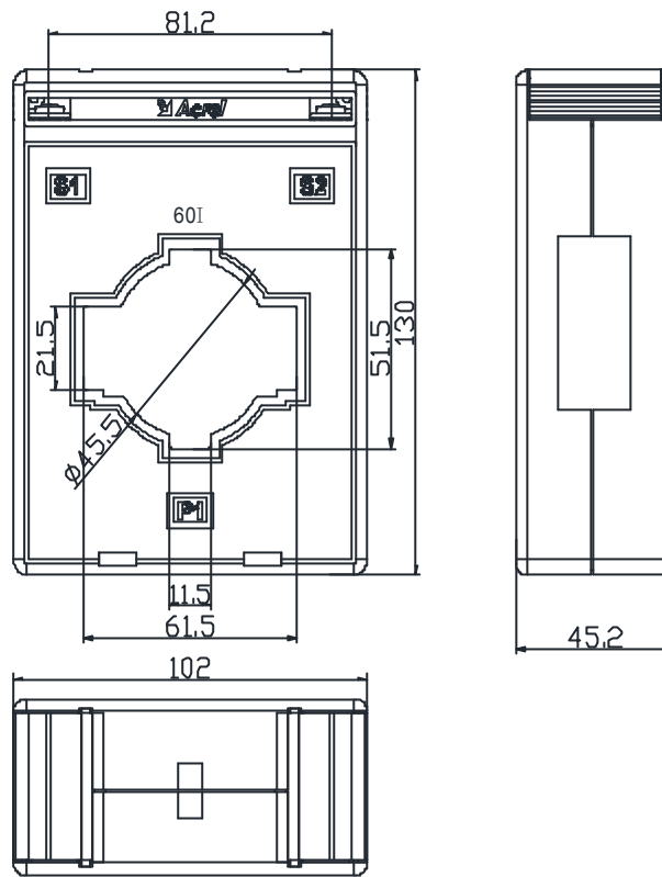
图 7 400A 电流互感器外形尺寸 Figure 7 Outline drawing of 400A current transformer
