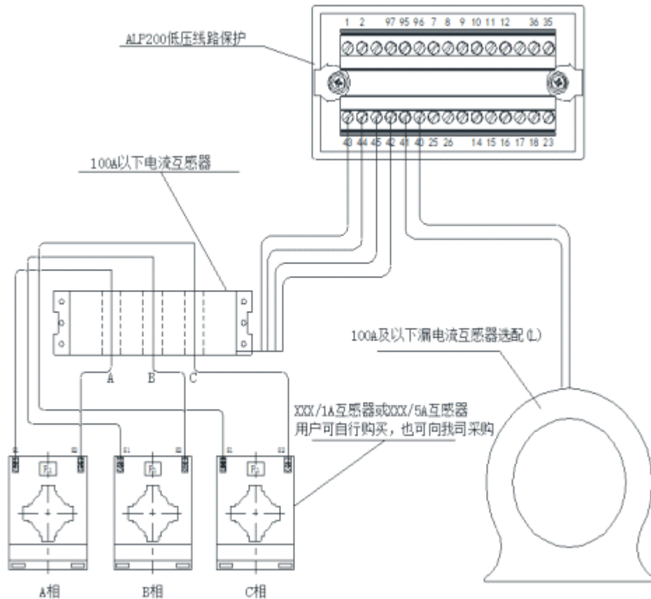
图 12 ALP200-1A、ALP200-5A 产品组成 Figure 12 Product composition of ALP200-1A, ALP200-5A
